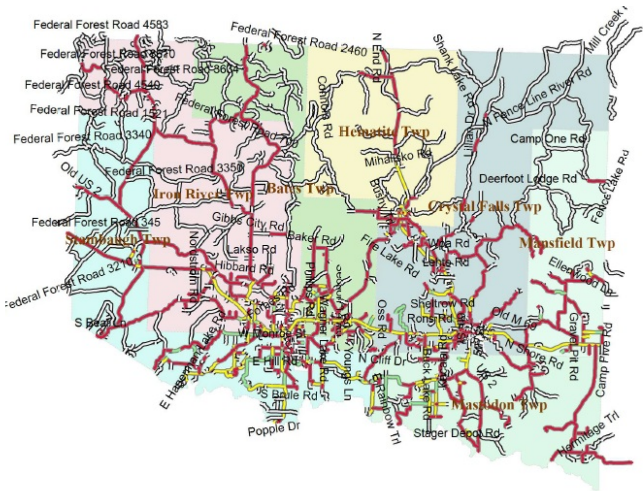
Figure 16: Map of the current paved road condition in good (PASER 10, 9, 8) shown in green, fair (PASER 7, 6, 5) shown in yellow, and poor (PASER 4, 3, 2, 1) shown in brown. Only Roads owned by ICRC are shown.
