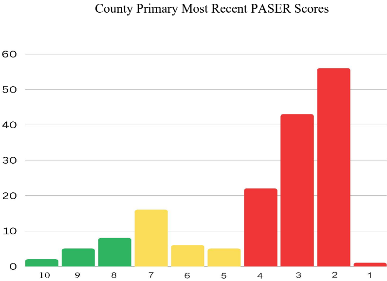
Figure 13: ICRC paved county primary road network conditions. Bar graph colors correspond to good/fair/poor TAMC designations.
