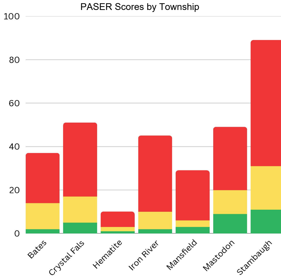
Figure 15: Number of miles of paved road in each township divided in categories of good (PASER 10, 9, 8), fair (PASER 7, 6, 5), and poor (PASER 4, 3, 2, 1). Only newly paved roads have been entered and the local system since 2000 and has not been PASER rated since.
